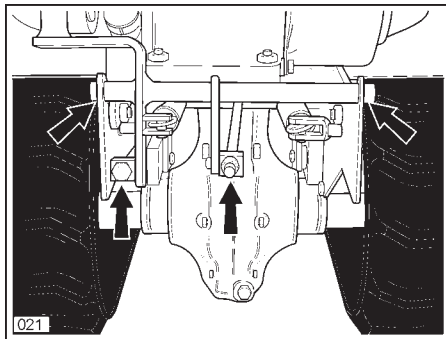
Brake lever pins
