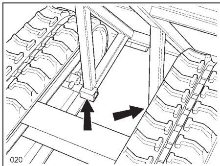
Box Support
