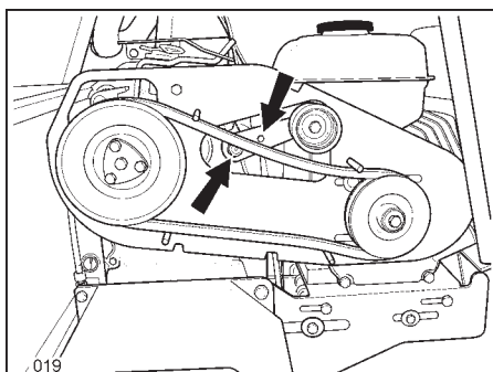
Tensor correia
