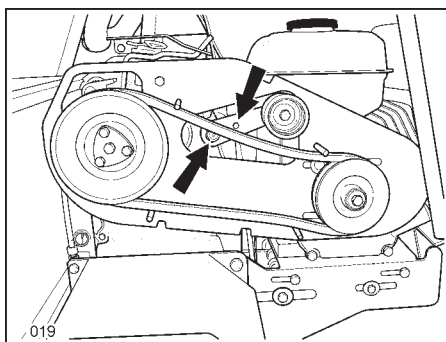
Belt tightener
